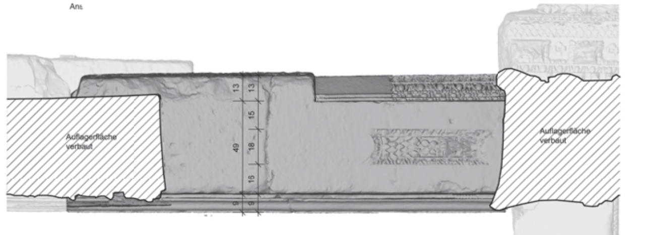
Architrav 100A
